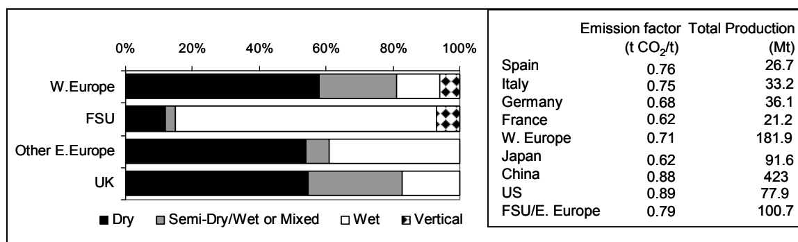
Figure 5 Kiln Type (%) and production for cement, by region
